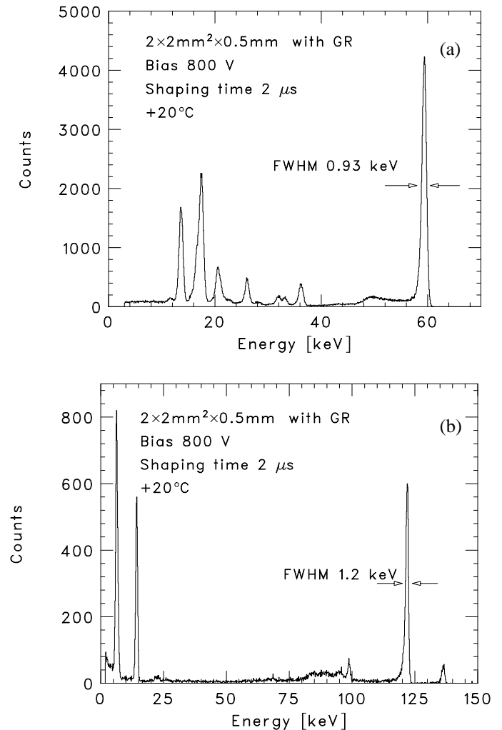
Fig. 6. (a) ^{241}\text{Am} and (b) ^{57}\text{Co} spectra obtained using a guard-ring CdTe diode with an active area of 2 \times 2 \text{ mm}^2 and a thickness of 0.5 mm.
