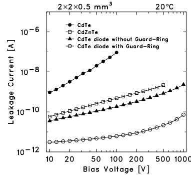
Fig. 2. Current-voltage (I-V) characteristics of CdZnTe and CdTe detectors with dimensions of 2 \times 2 \times 0.5 \text{ mm}^3 measured at 20^\circ\text{C} . For the guard ring device, the central active area is 2 \times 2 \text{ mm}^2 and the width of the guard ring around it is 500 \mu\text{m} . The gap between the active area and the guard ring is 50 \mu\text{m} .
